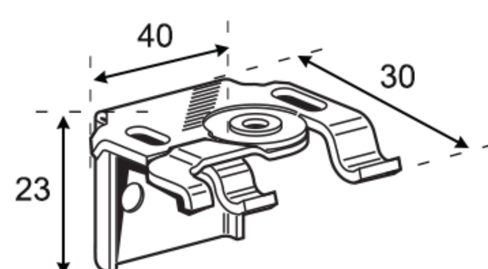
Support standard invisible
